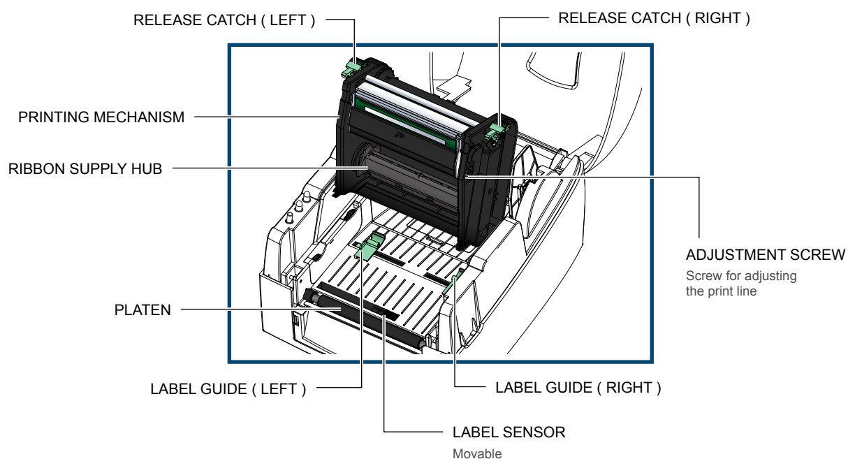
Barcode Printer
